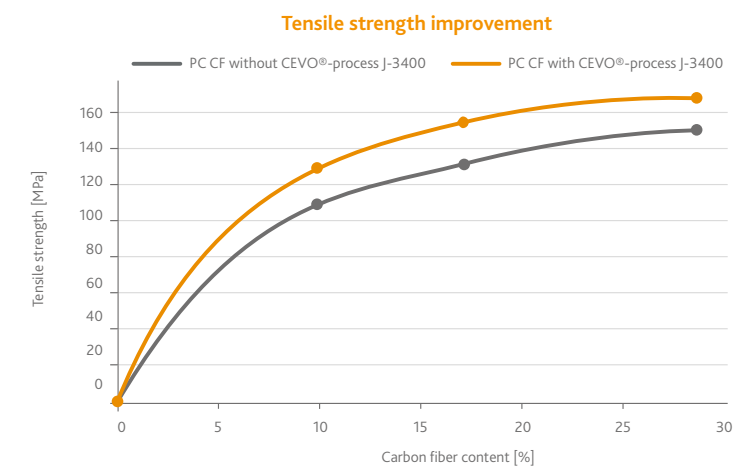
Figure 9: Effect of the inclusion of 0.3 phr of CEVO®-process J-3400 on tensile strength of PC reinforced with carbon fibre contents of 9.7, 17.2 and 28.5 phr
