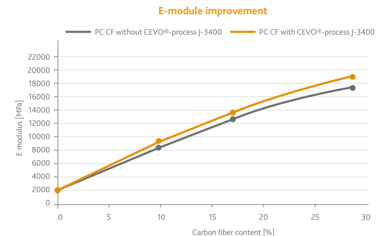
Figure 8: Effect of the inclusion of 0.3 phr of CEVO®-process J-3400 on tensile (E) modulus of PC reinforced with carbon fibre contents of 9.7, 17.2 and 28.5 phr
